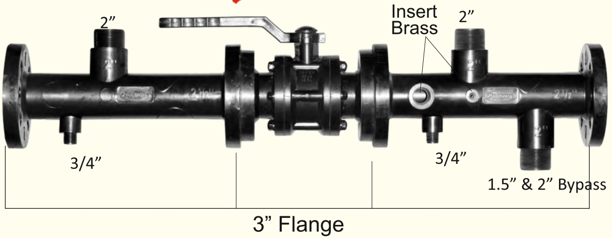
Header Flanged 2.1/2" & 3" Set with Ball Valve
